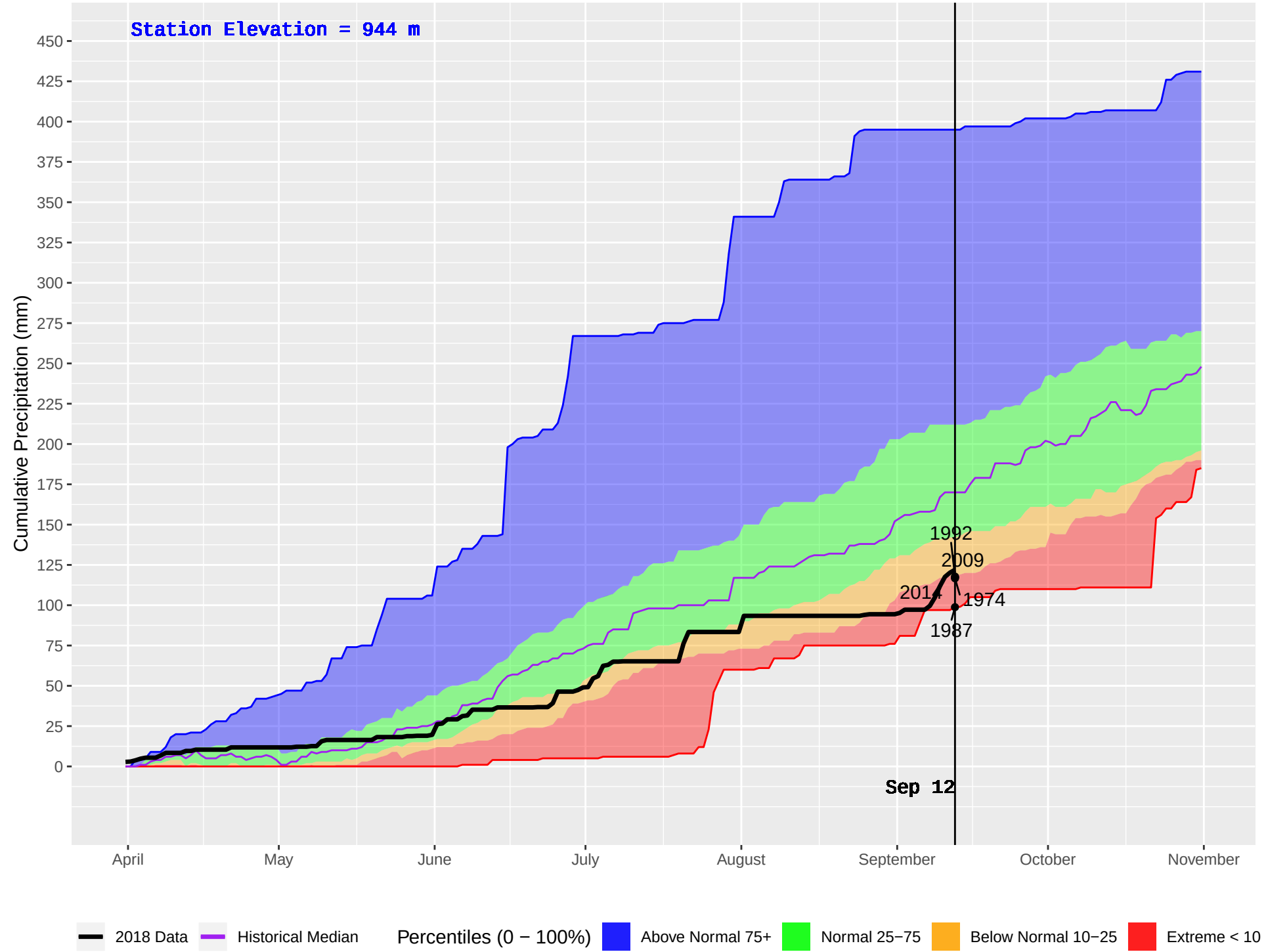
GRASSY PLAINS HUB (161) : Historical (1970–2016) and Current (2018) Daily Cumulative Precipitation
