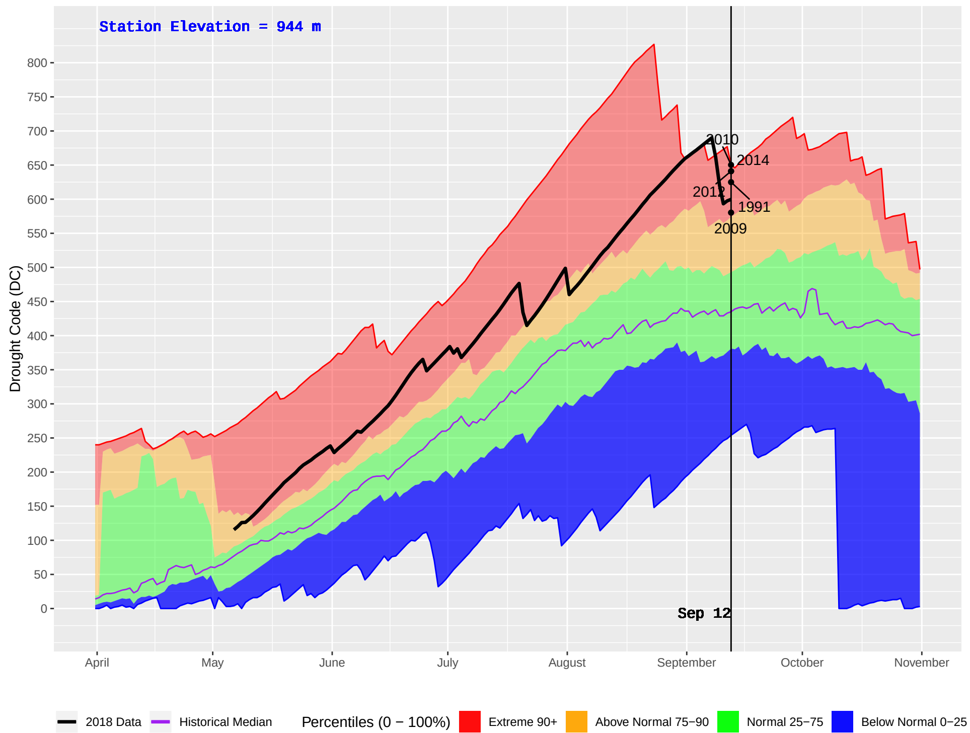
GRASSY PLAINS HUB (161) : Historical (1970–2016) and Current (2018) Daily Drought Code (DC)
