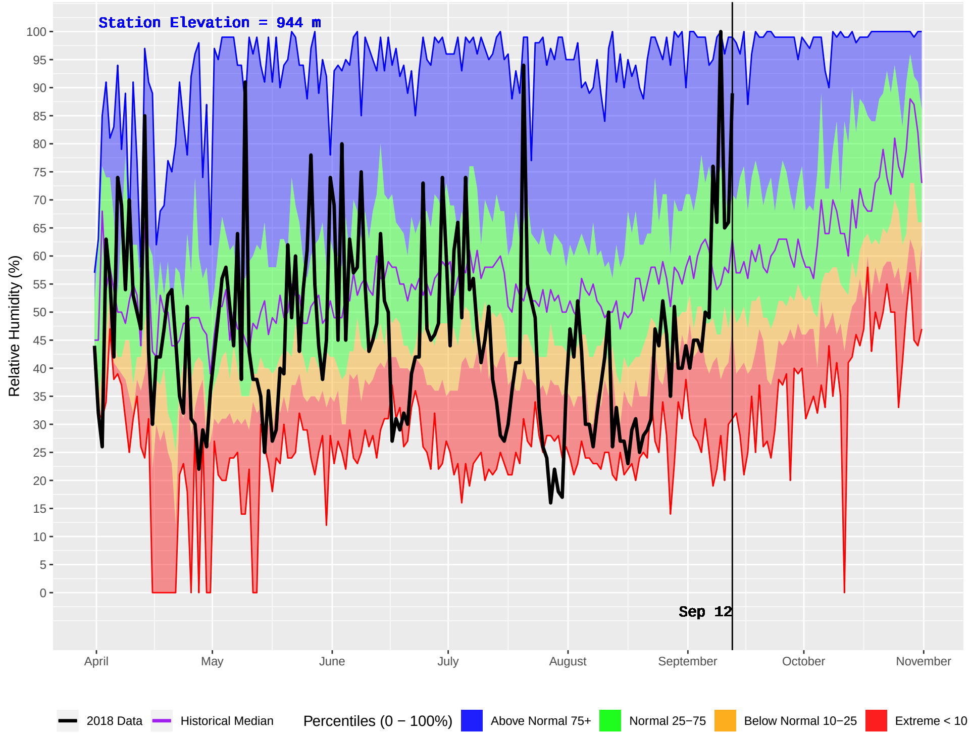
GRASSY PLAINS HUB (161) : Historical (1970–2016) and Current (2018) Daily Relative Humidity
