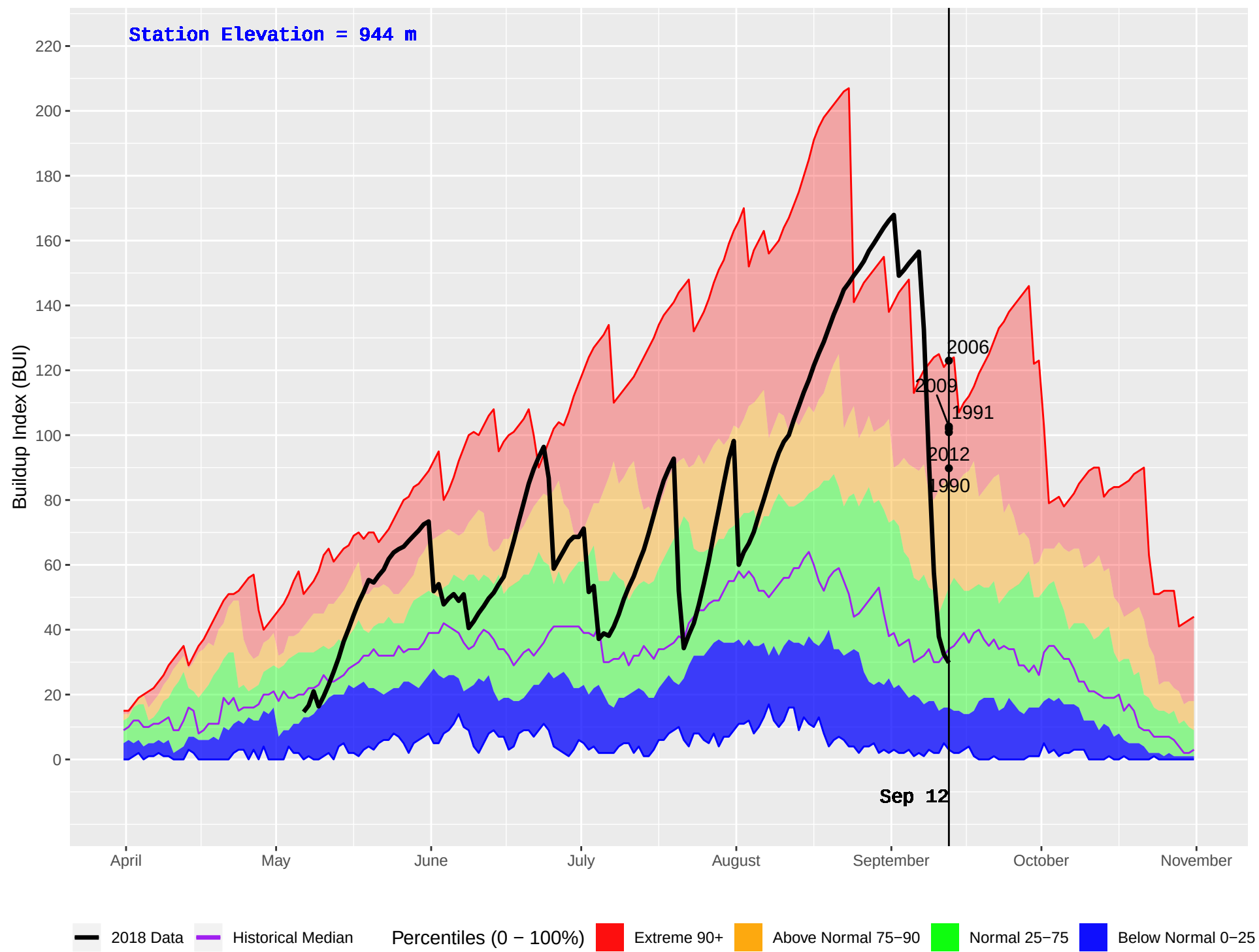
GRASSY PLAINS HUB (161) : Historical (1970–2016) and Current (2018) Daily Buildup Index (BUI)
