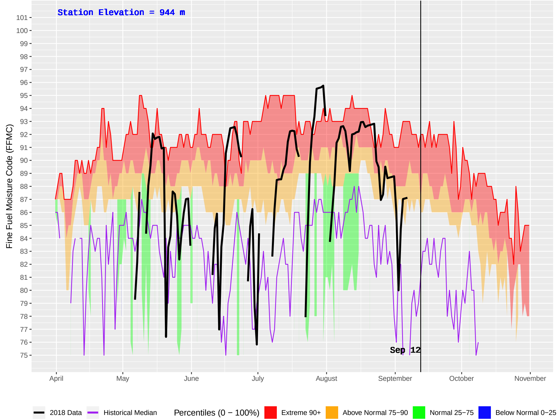
GRASSY PLAINS HUB (161) : Historical (1970–2016) and Current (2018) Daily Fine Fuel Moisture Code (FFMC)
