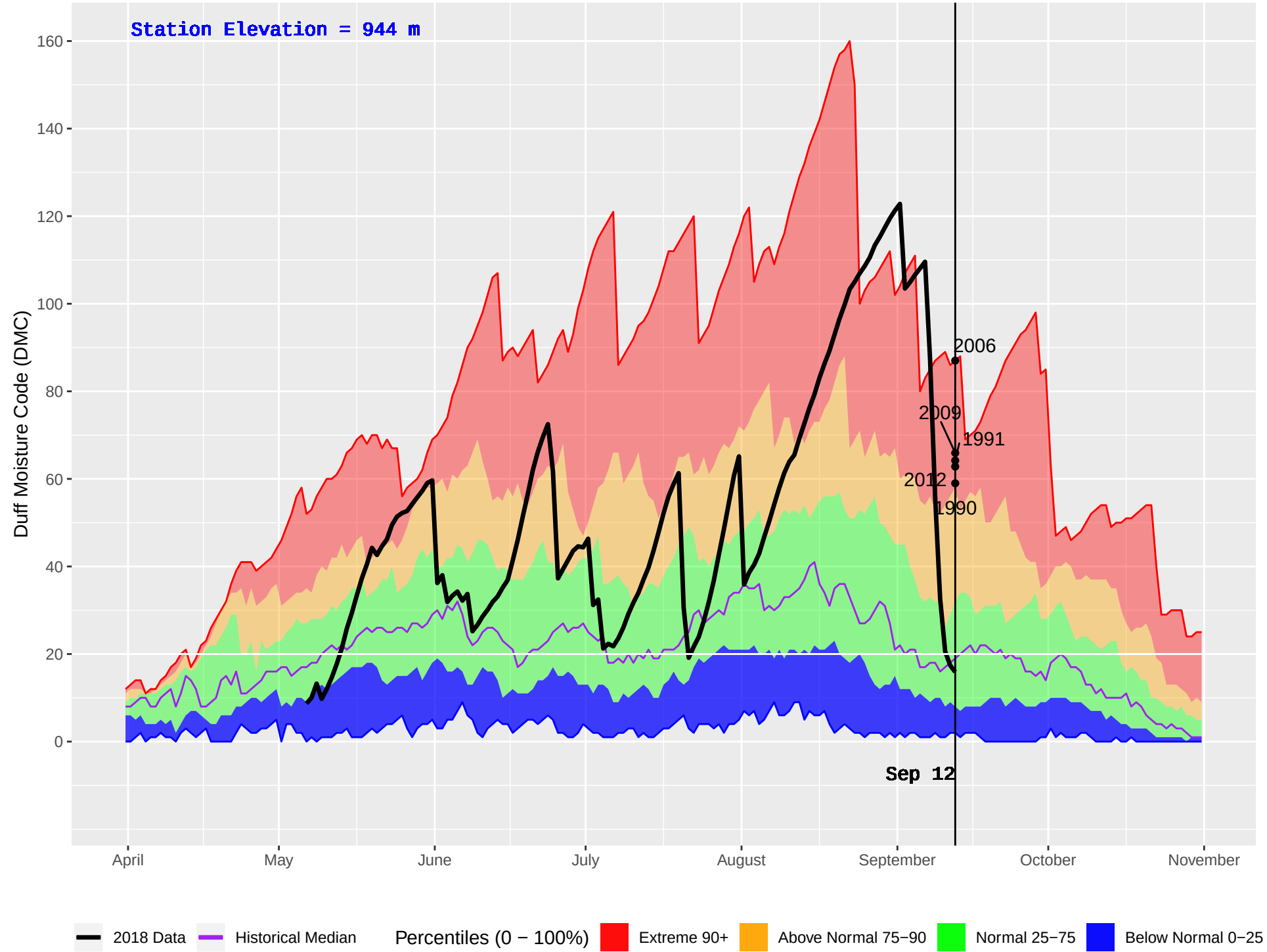
GRASSY PLAINS HUB (161) : Historical (1970–2016) and Current (2018) Daily Duff Moisture Code (DMC)
